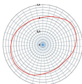
Horizontal Polarization
