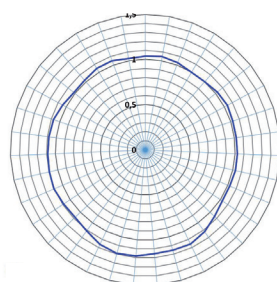
Vertical Polarization
